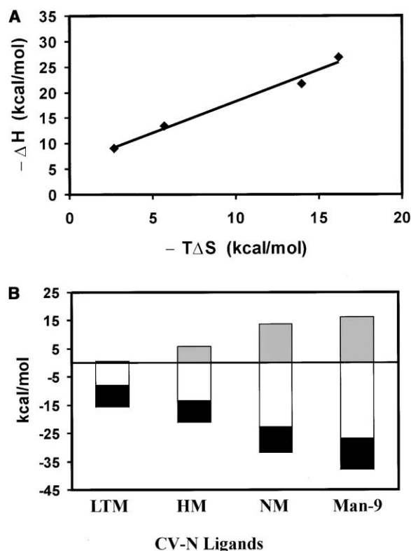
Figure 3. Enthalpy-Entropy Compensation
